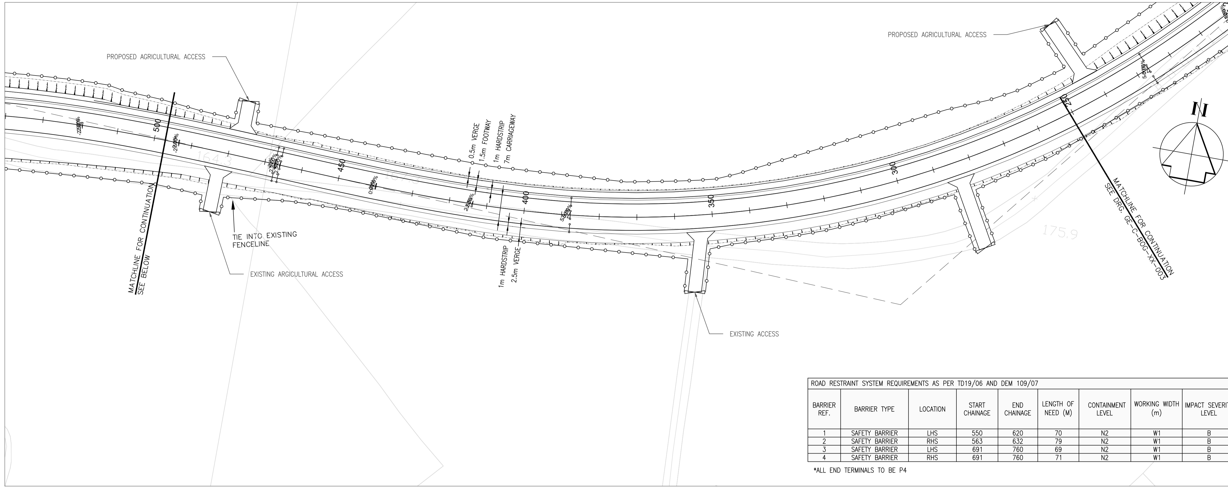
PROPOSED BOGHILL ROAD PLAN (250m-500m) (SCALE 1:500)
