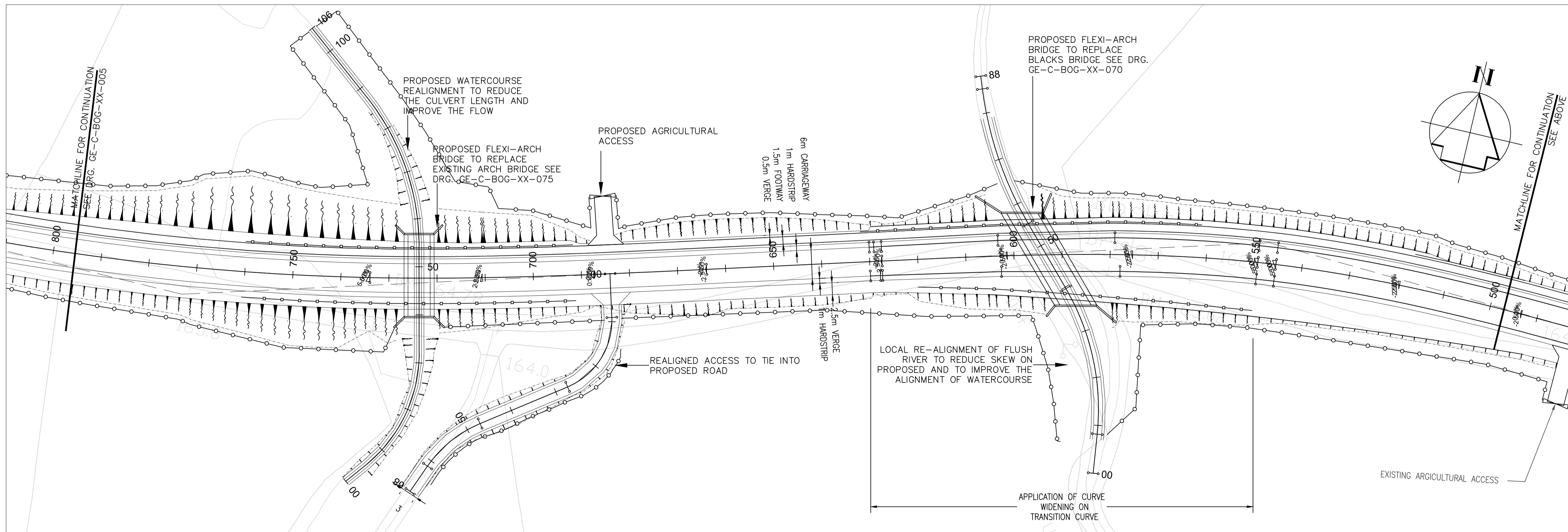
PROPOSED BOGHILL ROAD PLAN (500m-800m) (SCALE 1:500)
