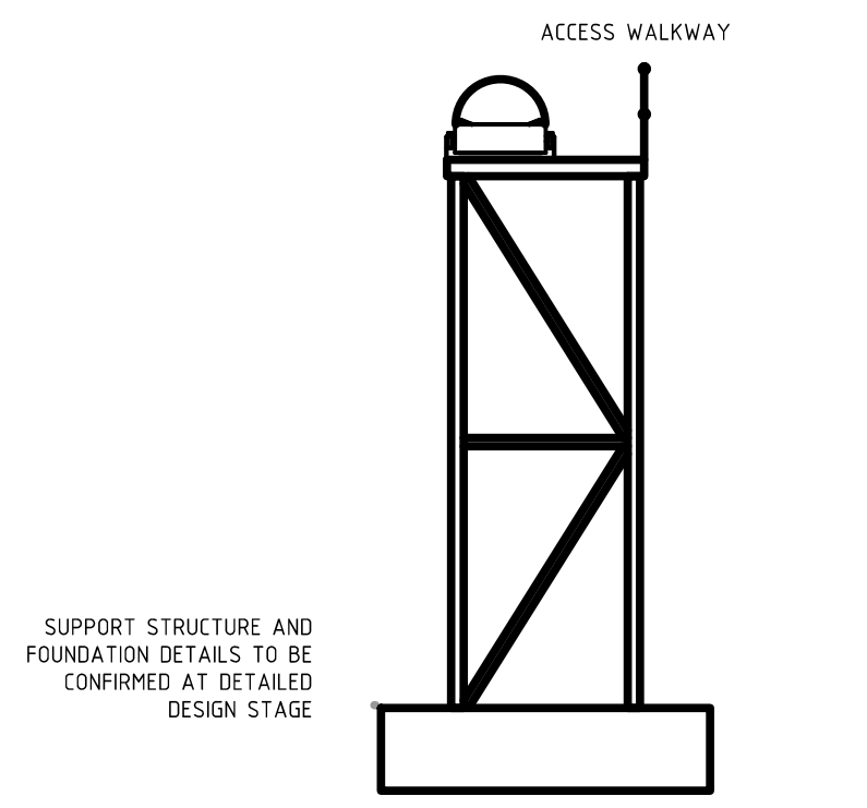
TYPICAL CROSS SECTION 1:100
