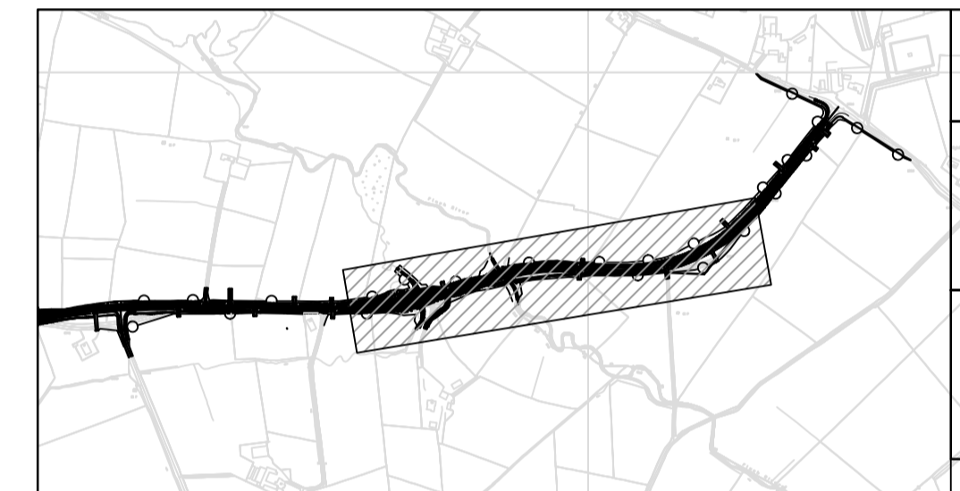
KEYPLAN (NTS)
